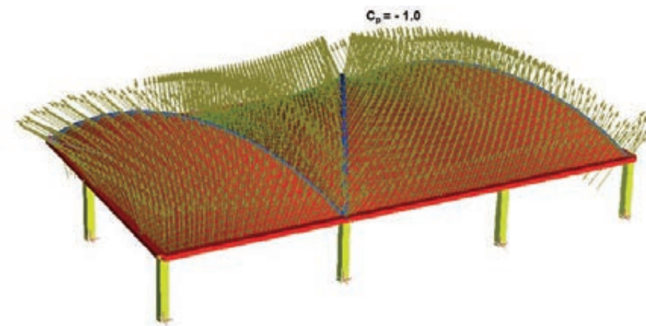
Wind load
